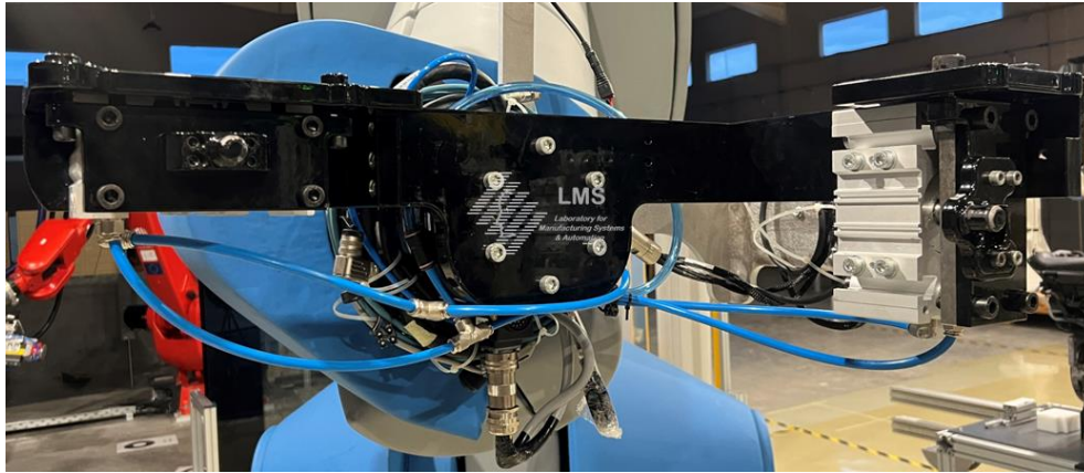
Figure 10: Gearbox gripper
