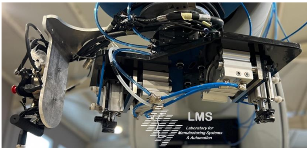
Figure 9: Motor gripper
